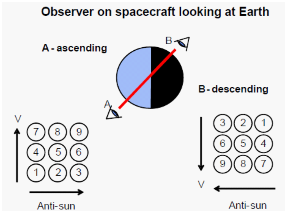
Figure: 6.2-1 CrIS Field of Regard
